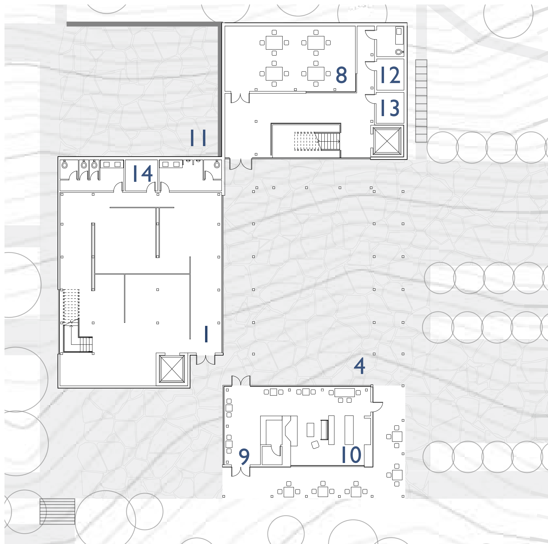
Ground Plan
