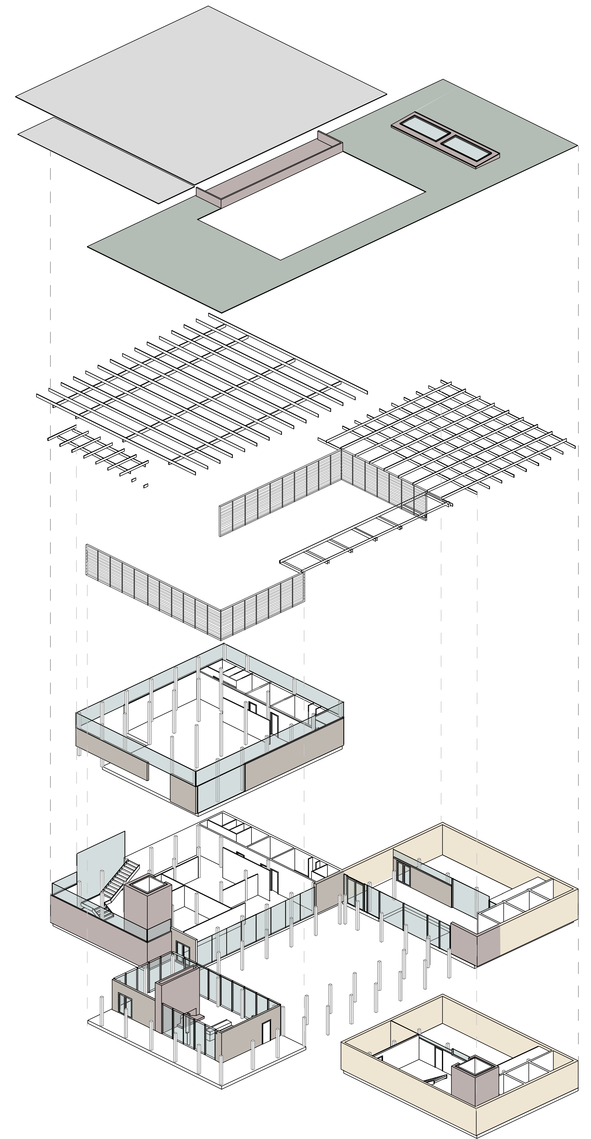
Exploded Axonometric
