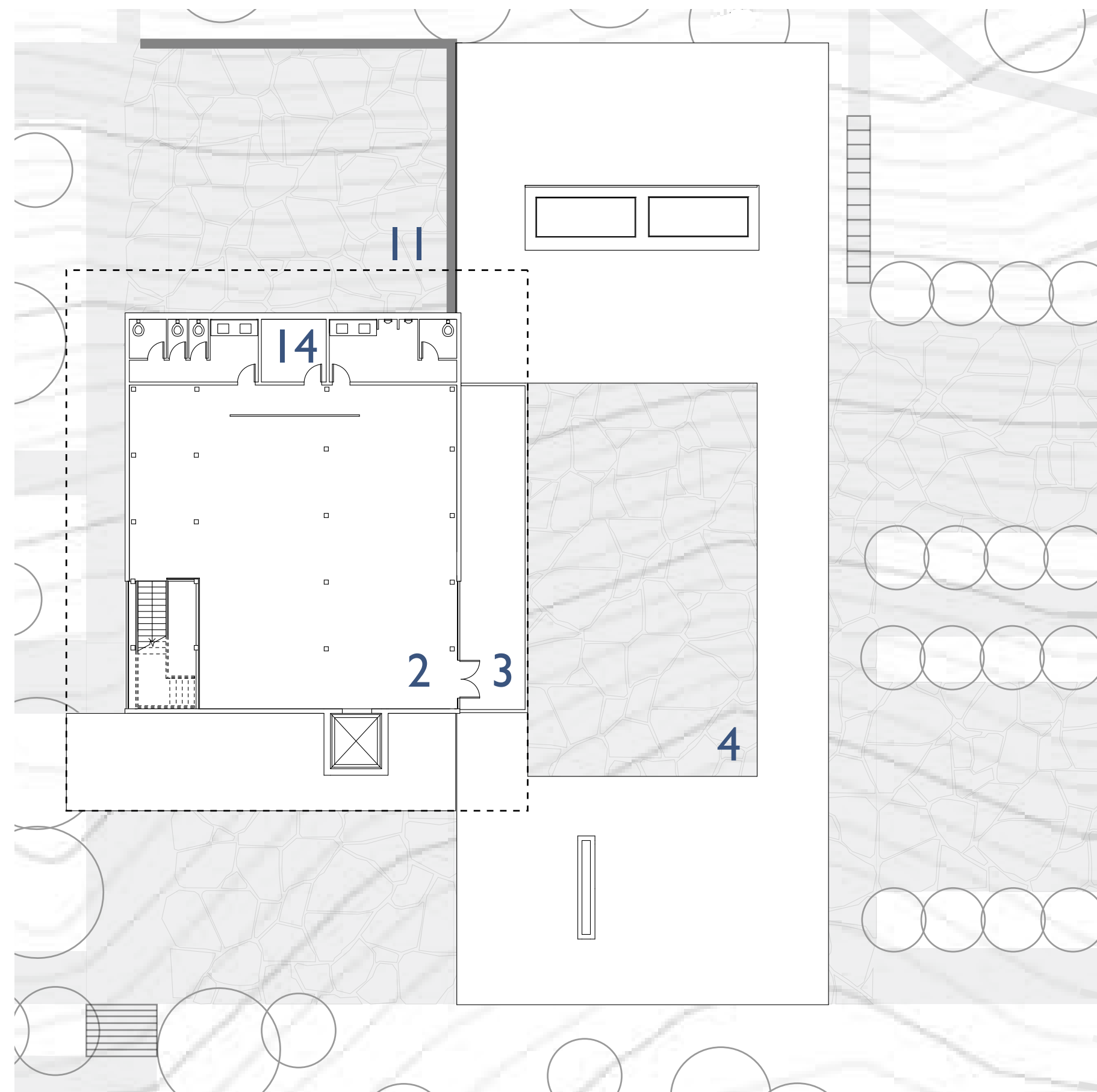
Upper Level Floor Plan
