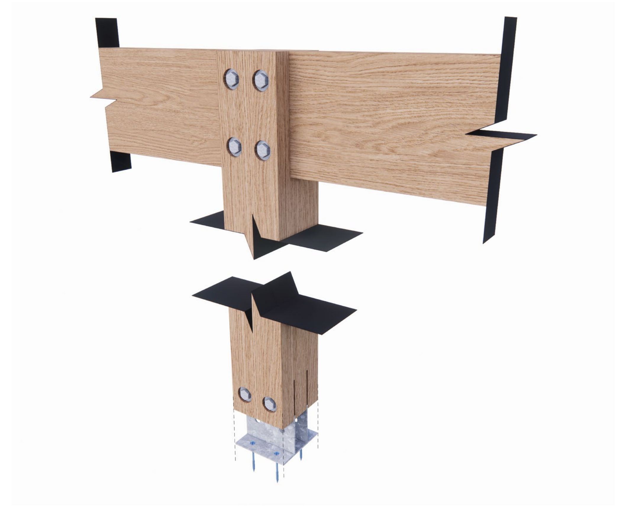
Column Beam Connections
